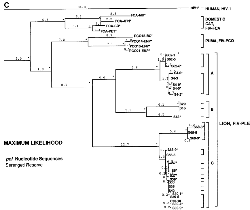
FIG. 4. Evolutionary trees of the 28 Serengeti FIV-Ple sequences from 15 lions and other feline and human lentivirus pol genes. Sequences were aligned as described in Materials and Methods. (a) Neighbor-joining phenetic tree using distance matrix as described in the legend to Fig. 3 (45). Branch lengths reflect percent nucleotide divergence. In parentheses are the numbers of bootstrap iterations (of 100) that support the adjacent node. (b) PAUP maximum parsimony tree (50). The strict bootstrap consensus tree presented here has an overall length of 580 changes and a consistency index of 0.65, yielding a 35% convergence level. The scale and branch lengths are presented as the number of nucleotide substitutions (preceding the slash) with the number of unambiguous substitutions (following the slash). An unambiguous site is equivalent to the branch length minus the homoplasy. Bootstrap values (of 100 iterations) are in parentheses. (c) Maximum likelihood tree from DNAML (14). This tree phylogeny was based on the most statistically significant tree of 12,609 trees examined. This tree was generated using a transition/transversion ratio of 2. Branch lengths are substitutions, relative to the tree shown, shown as 100 times the expected number of substitutions per site. Branch lengths not significantly different from zero were collapsed into polytomies. Asterisks indicate significant support ( P \leq 0.01 ) for adjacent divergence node. The ln likelihood for the presented tree is -3,217.38 . See legend to Fig. 3 for geographic and virus abbreviations.
