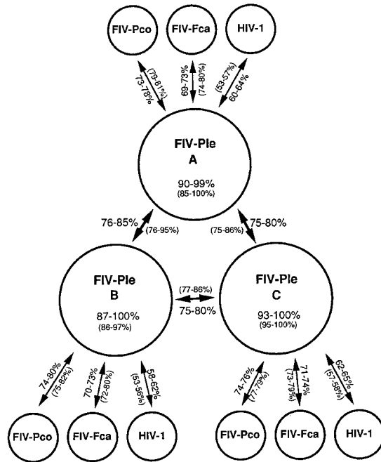
FIG. 5. Schematic showing the minimum and maximum percent nucleotide sequence identities within and between the three major FIV-Ple clades as well as between the FIV-Ple clades and other feline and human lentiviruses. The clade letter designations of the three FIV-Ple clades are present within the large circles (A, B, and C). Minimum-maximum percent sequence identities within each of the three FIV-Ple clades are listed within each clade. Minimum-maximum percent sequence identities between various clades or species are listed along the arrows that designate the viruses being compared. Minimum and maximum percent amino acid similarities are also listed in parentheses within clades, between clades, and between feline and human lentiviruses. Virus abbreviations are as listed in the legend to Fig. 3.
